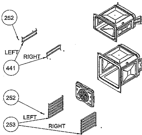
CAVITY ASSEMBLY WITH WIRE SHELF (OPTIONAL)
