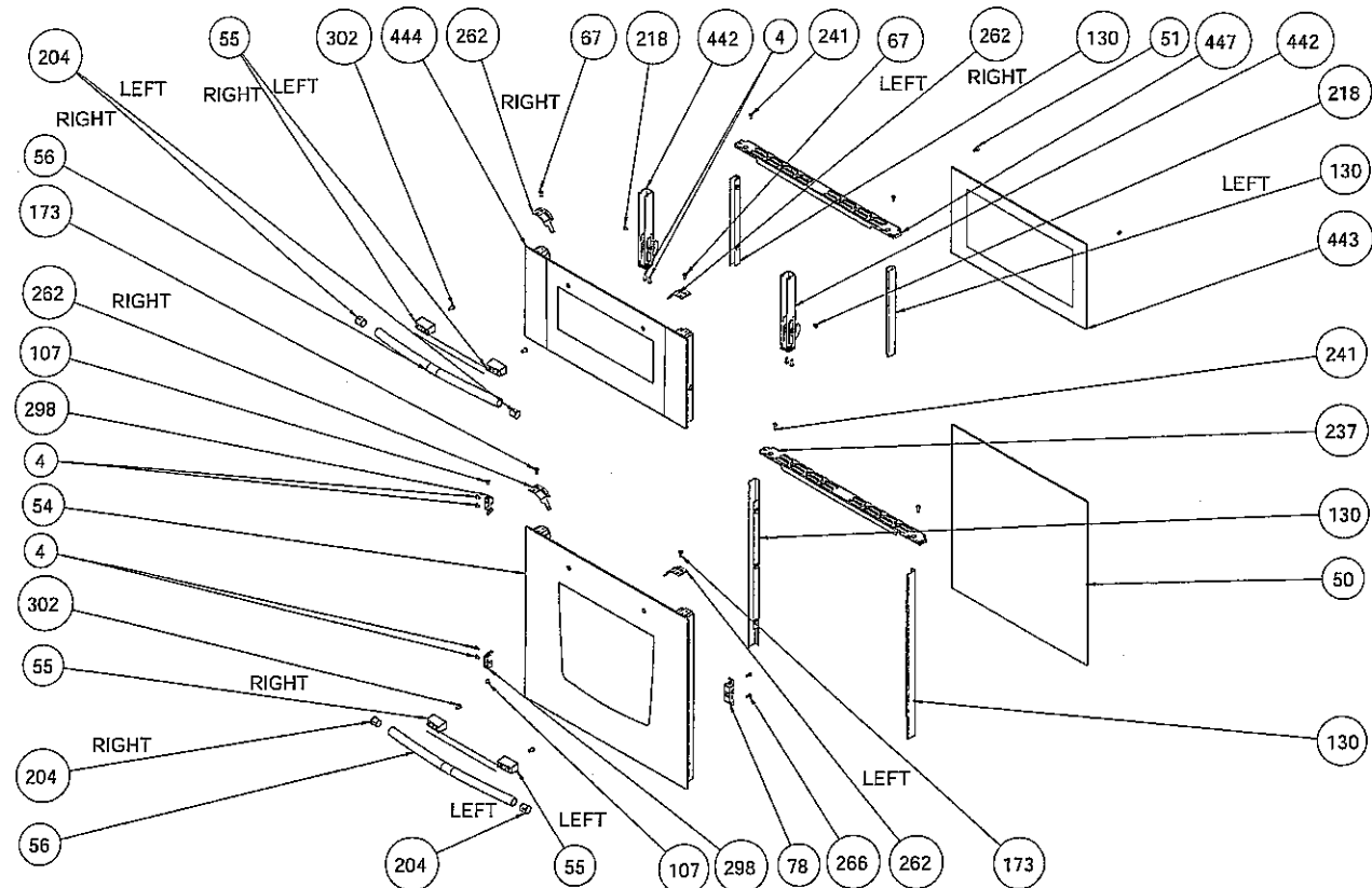
FLAT TYPE - SIDE OPENING OVEN DOOR (OPTIONAL) (POSITION NO 377)
