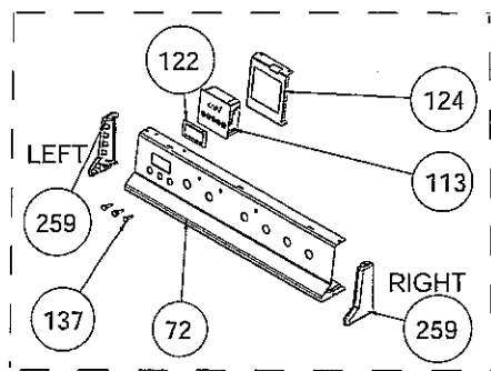
60X60 DIGITAL TIMER (OPTIONAL)
