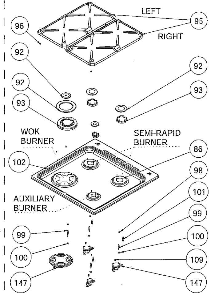
3 GAS + WOK BURNER
