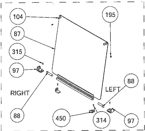
GLASS LID WITH BUMPER OPTIONAL
