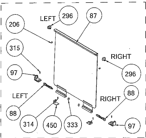
GLASS LID WITH SHORT PROFILE OPTIONAL
