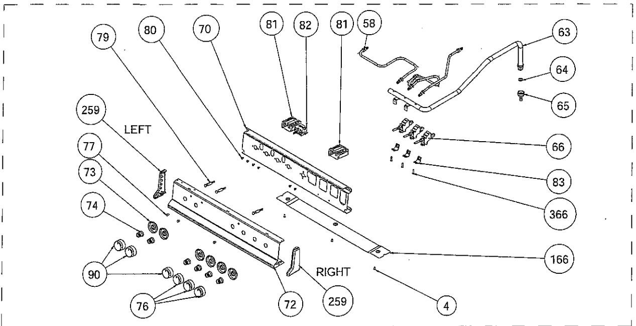
3G-1E CONTROL PANEL ASSEMBLY
